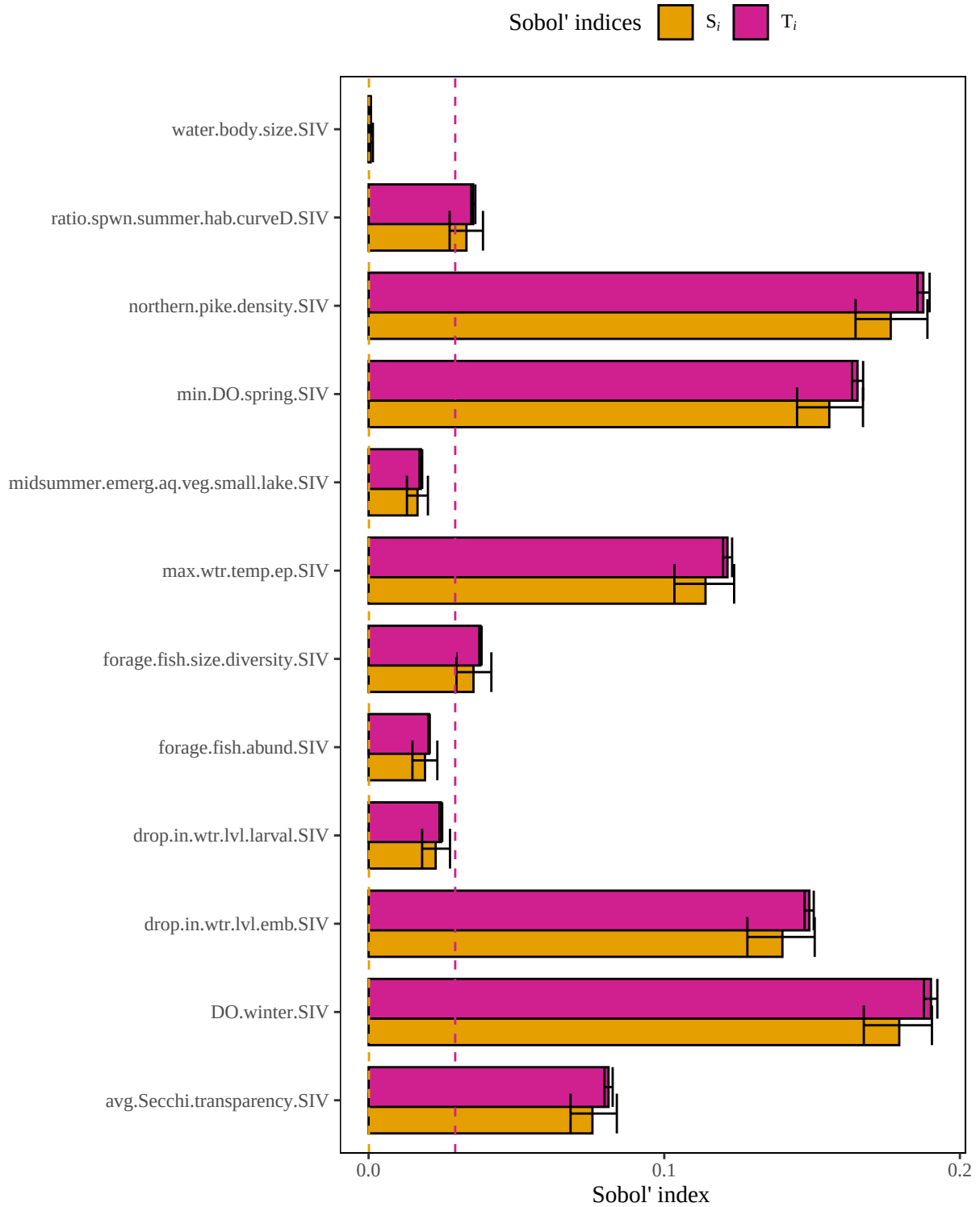
Figure 5. Results of a sensitivity analysis for the muskellungeSmallLakeSpwnVegCurveD model based on a geometric mean structure. Dashed lines represent baseline numerical approximation error for S_i and T_i ( i.e. , dummy variables).
